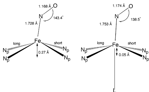
Figure 7. Comparison of structural parameters for \langle[\text{Fe}(\text{Por})(\text{NO})]\rangle and \langle[\text{Fe}(\text{Por})(\text{NO})(\text{L})]\rangle , representative geometries for the five- and six-coordinate \{\text{FeNO}\}^7 porphyrinate systems. Values are taken from Table 2.
