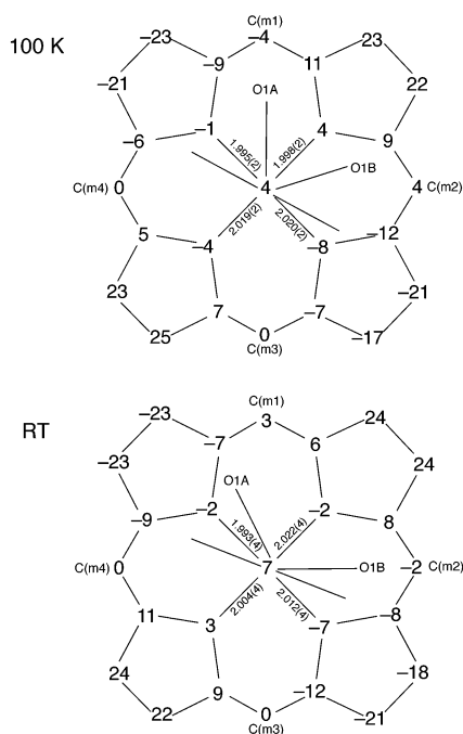
Figure 5. Formal diagram of the porphyrinato core of [Fe(TPP)(NO)(1-MeIm)], at 100 K (top) and room temperature (bottom), displaying the perpendicular displacements (in units of 0.01 Å) of the core atoms from the 24-atom mean porphyrin plane. Positive displacements are toward the nitrosyl-coordinated face of the porphyrin. The projections of the two axial ligands are shown. The major orientation of the nitrosyl oxygen at both temperatures is denoted as O1A. Data at room temperature are taken from ref 8.
