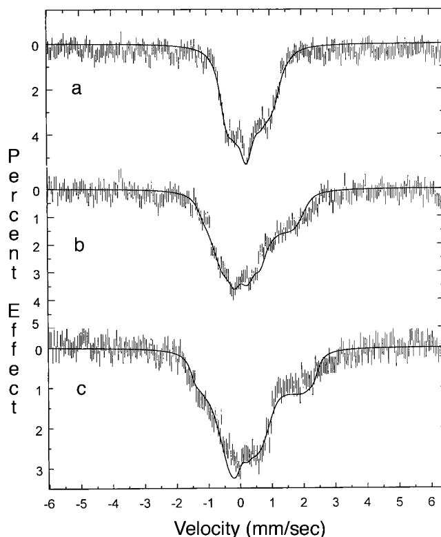
Figure 8. Mössbauer spectra of [\text{Fe}(\text{TPP})(\text{NO})(1\text{-MeIm})] at 4.2 K in an applied field of (a) 3 T, (b) 6 T, and (c) 8.8 T parallel to the \gamma -ray beam. The solid lines are simultaneous fits to the three spectra without rotation of the EFG tensor. The parameters determined by these fits are listed in Table 5.
