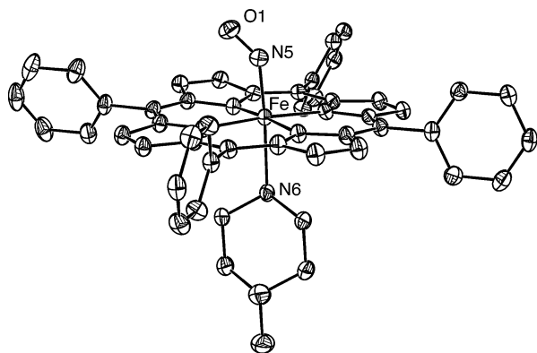
Figure 4. ORTEP diagram of [Fe(TPP)(NO)(4-MePip)] with 50% probability ellipsoids.
