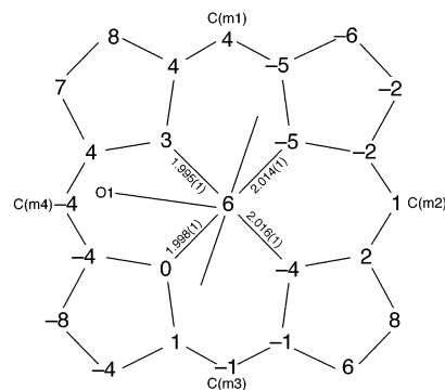
Figure 2. Formal diagram of the porphyrinato core of [Fe(TPP)(NO)(4-NMe 2 Py)] displaying the perpendicular displacements (in units of 0.01 Å) of the core atoms from the 24-atom mean porphyrin plane. Positive displacements are toward the nitrosyl-coordinated face of the porphyrin. The projections of the two axial ligands are shown.
