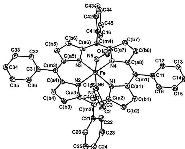
Figure 3. ORTEP diagram of [Fe(TPP)(NO)(1-MeIm)] with 50% probability ellipsoids. The labeling scheme for the porphyrin core is also shown.
