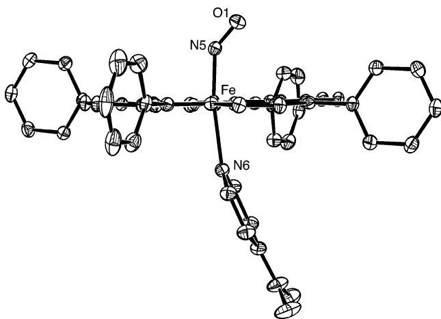
Figure 1. ORTEP diagram of [Fe(TPP)(NO)(4-NMe 2 Py)] with 50% probability ellipsoids.
