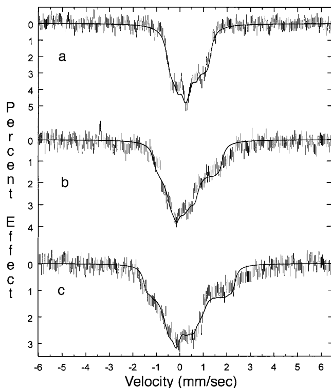
Figure 9. Mössbauer spectra of [\text{Fe}(\text{TPP})(\text{NO})(1\text{-MeIm})] at 4.2 K in an applied field of (a) 3 T, (b) 6 T, and (c) 8.8 T parallel to the \gamma -ray beam. The solid lines are simultaneous fits to the three spectra, including Euler angles ( \alpha ) and ( \beta ) to model rotation of the EFG tensor. The parameters determined by these fits are listed in Table 5.
