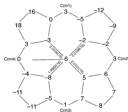
Figure 6. Formal diagram of the porphyrinato core of [Fe(TPP)(NO)(4-MePip)] displaying the perpendicular displacements (in units of 0.01 Å) of the core atoms from the 24-atom mean porphyrin plane. Positive displacements are toward the nitrosyl coordinated face of the porphyrin. The projection of the nitrosyl ligand is shown.
